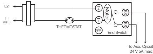
Figure-1 Typical Wiring of a PopTop to Replace a Honeywell Valve.
