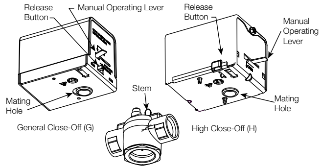
Figure-7 PopTop Installation.
