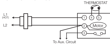
Kele Wire Leads
