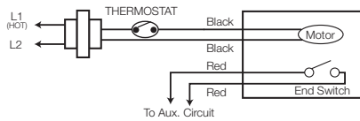
Kele Wire Leads
