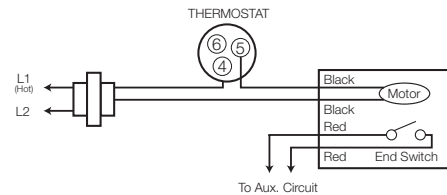
Kele Wire Leads
