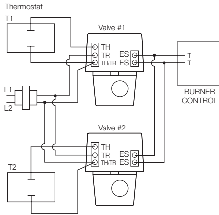
Figure-4 Typical Multiple Valve Wiring.
