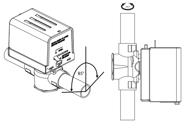
Figure-5 Mounting Position.
