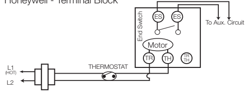
Honeywell - Terminal Block
