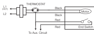
Kele Wire Leads
