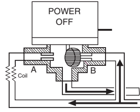
Figure-6d 3-Way Valve in Mixing Configuration Normally Open to the Coil.
